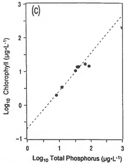
Figure 5.—Effect of data aggregation on the Chl-TP relation using data from Figure 3. a) Individual observations of Chl and TP from each lake. b) Seasonal mean values of Chl and TP for each lake. c) Lake mean values of Chl and TP. The dotted line on each panel is the lake mean regression from Figure 1c.
