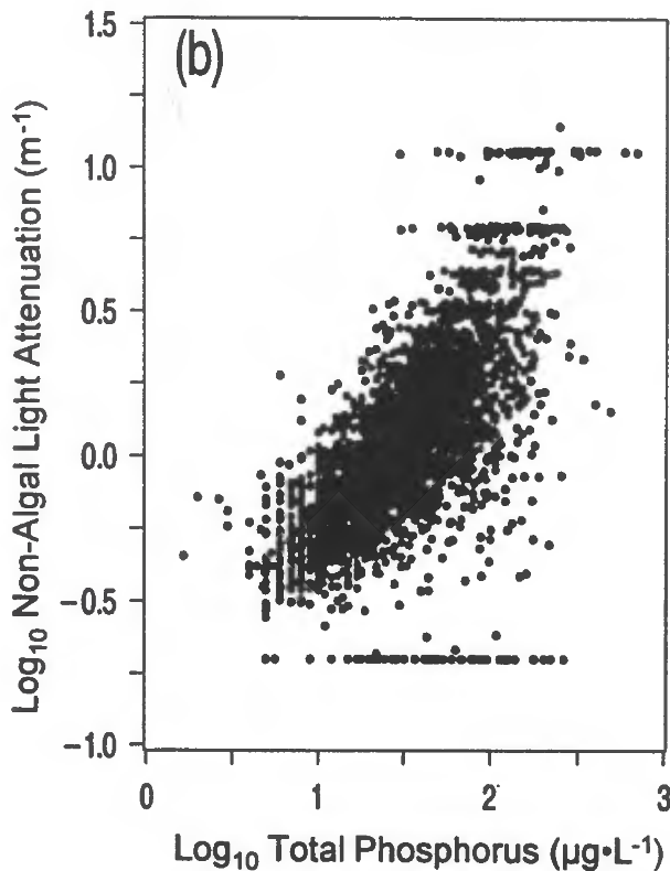
Figure 4.—Panel a. — Plot of non-volatile suspended solids (mg/L) in individual samples against TP in the same sample. Panel b. — Plot of non-algal light attenuation ( K_{na} ) against TP.
